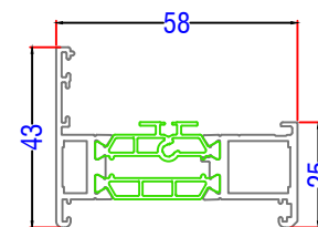
U44008 - Outer Frame
