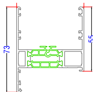
U44012- Deep Outer Frame
