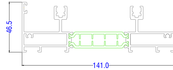
U11028 - Duo Frame Threshold
