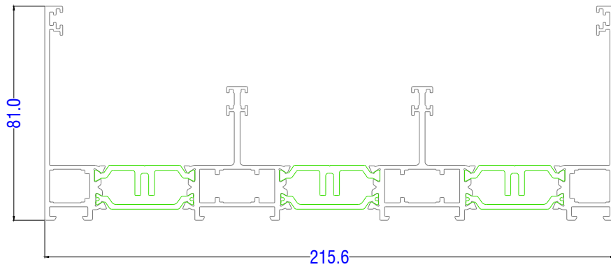
U11064 - Tri Frame
