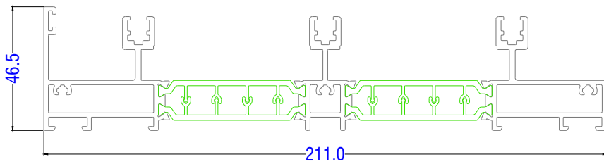
U11065 - Tri Frame Threshold
